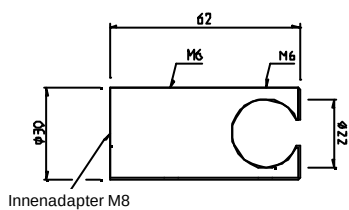
Innenadapter M8
