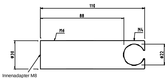
Innenadapter M8
